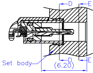
RECOMMENDED SET BODY SIDE HOLE SHAPE
