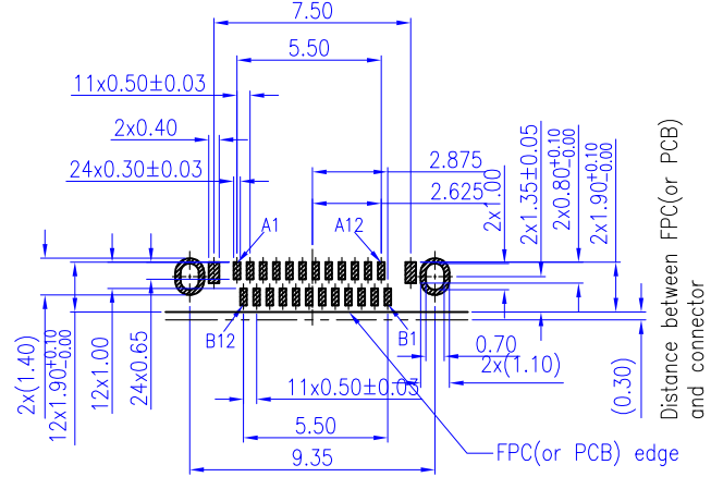
RECOMMENDED PCB LAYOUT DEFAULT TOLERANCE:±0.05
